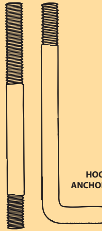
HIGHWAY ANCHOR BOLT (STREET LIGHT)
